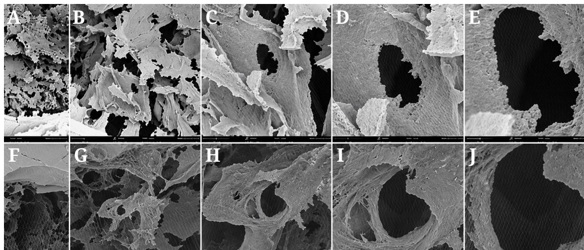
Figure 7. SEM images of water-soluble chitosan-tripolyphosphate (CS-TPP) cross-section in (A) 300x, (B) 1000x, (C) 3000x, (D) 6000x, and (E) 12000x magnification; and garlic peel polyphenol (GPP)-encapsulated CS-TPP matrices (GPP@CS-TPP) cross-section in (F) 300x, (G) 1000x, (H) 3000x, (I) 6000x, and (J) 12000x magnification.
