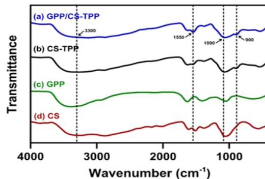
Figure 5. FTIR spectra of (a) garlic peel polyphenol (GPP)-encapsulated water-soluble chitosan-tripolyphosphate matrices (GPP@CS-TPP), (b) CS-TPP matrices, (c) GP, and (d) CS.
